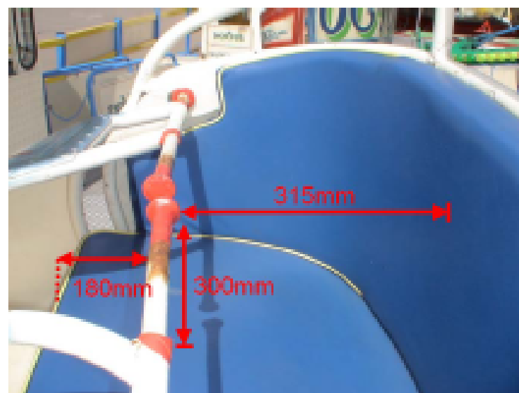
Photograph 5 Side view of the Octopus ride, showing the depth of the passenger seat and position of the containment, hand bar.
